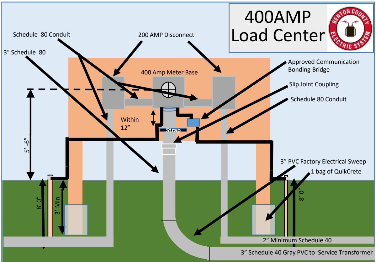
400 Amp Load Center
